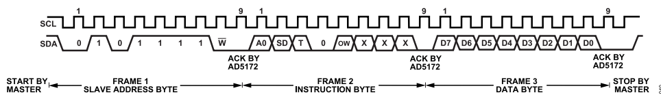
Figure 47. Writing to the RDAC Register—AD5172
