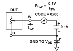
Figure 35. Incremental On Resistance
