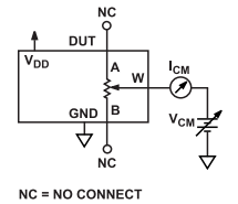
Figure 36. Common-Mode Leakage Current
