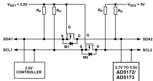
Figure 52. Level Shifting for Different Voltage Operation
