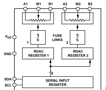
Figure 1. AD5172 Functional Block Diagram
