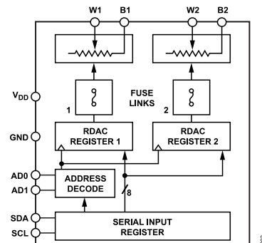
Figure 2. AD5173 Functional Block Diagram
