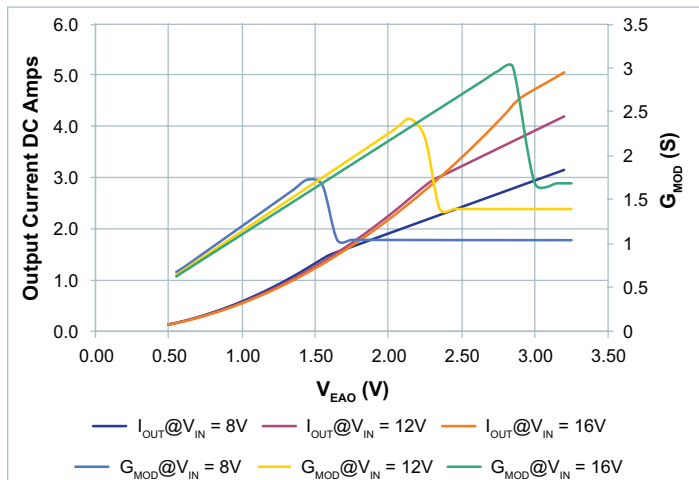
Figure 87 — G_{MOD} vs output current vs. V_{EAO} , V_{OUT} = 28\text{V} ; 8 – 16 V_{IN}
