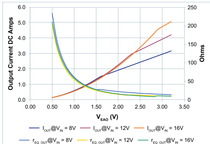
Figure 90 — r_{EQ\_OUT} vs. output current vs. V_{EAO} , V_{OUT} = 28\text{V} ; 8 – 16 V_{IN}
