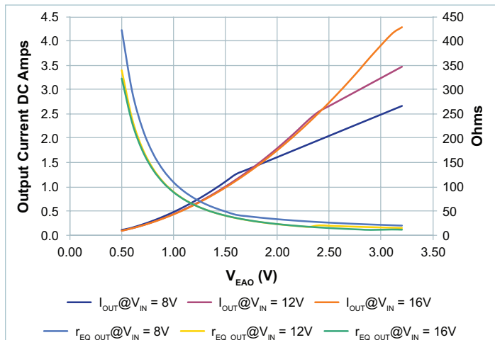
Figure 96 — r_{EQ\_OUT} vs. output current vs. V_{EAO} , V_{OUT} = 36\text{V} ; 8 - 16V_{IN}
