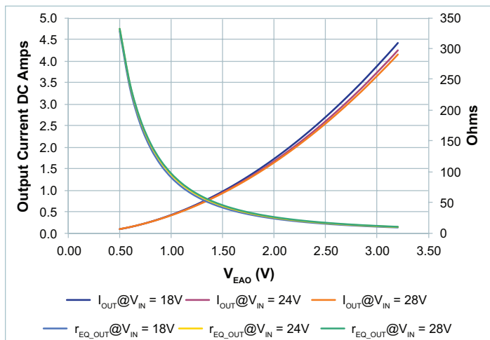
Figure 97 — r_{EQ\_OUT} vs. output current vs. V_{EAO} , V_{OUT} = 36\text{V} ; 18 - 28V_{IN}
