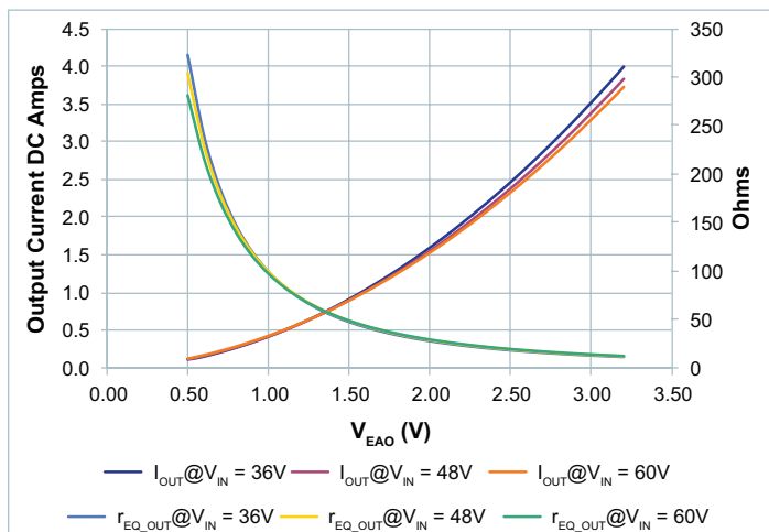
Figure 98 — r_{EQ\_OUT} vs. output current vs. V_{EAO} , V_{OUT} = 36\text{V} ; 36 - 60V_{IN}
