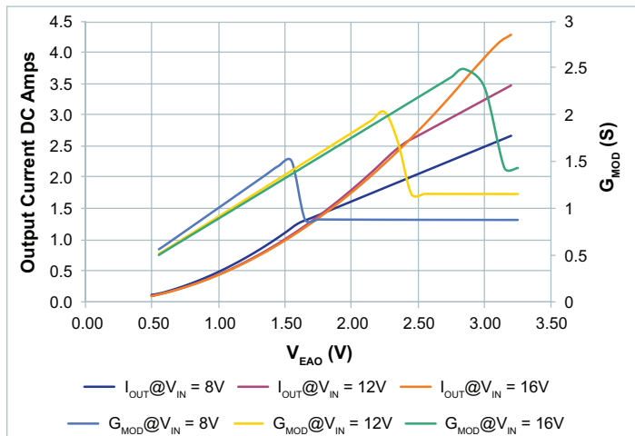
Figure 93 — G_{MOD} vs output current vs. V_{EAO} , V_{OUT} = 36\text{V} ; 8 - 16V_{IN}
