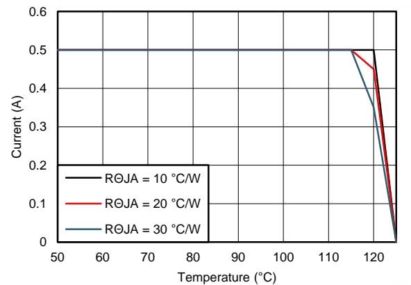
Figure 58. Derating Curve
