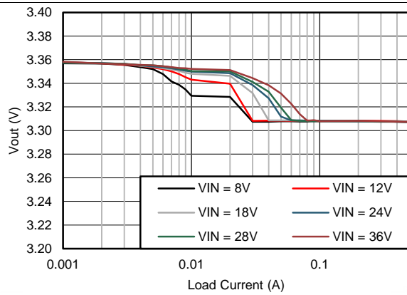
Figure 7. V_{OUT} Regulation
