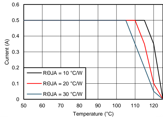
Figure 82. Derating Curve
