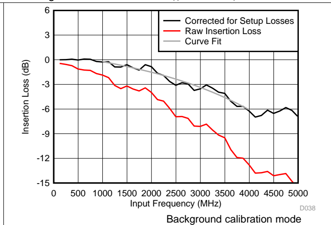
Figure 46. Insertion Loss vs Input Frequency
