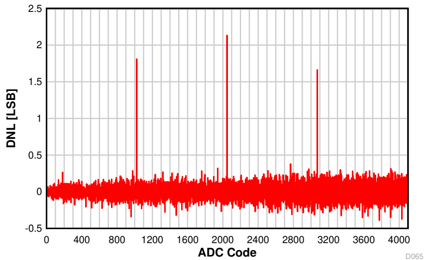
Figure 8-26. DNL vs. ADC Code
