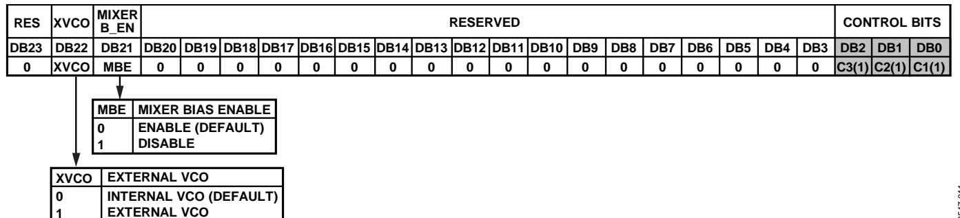
Figure 45. Register 7—Mixer Bias Enable and External VCO Enable Register Map
