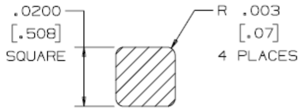
PIN CROSS SECTION
