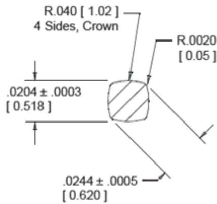
Pin Cross Section
