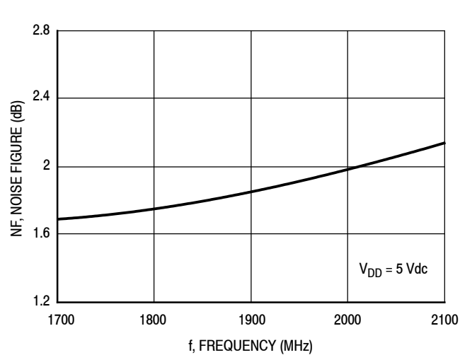
Figure 26. Noise Figure versus Frequency
