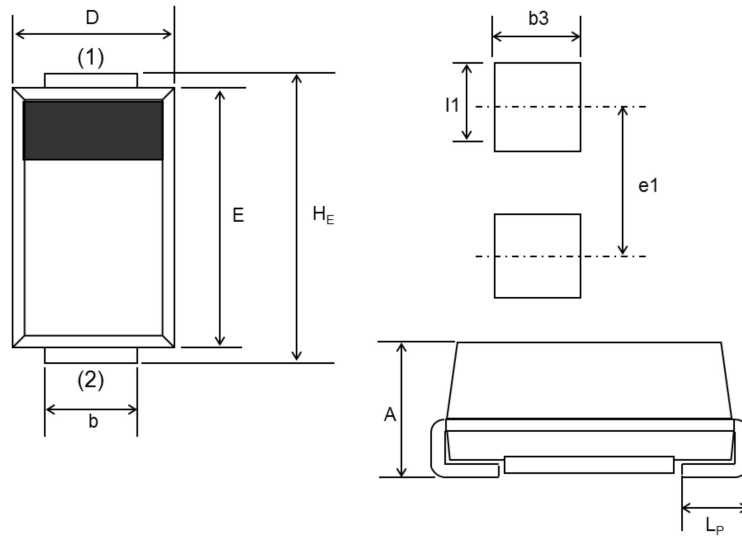
DO-214AC(SMA), (FVDS)
