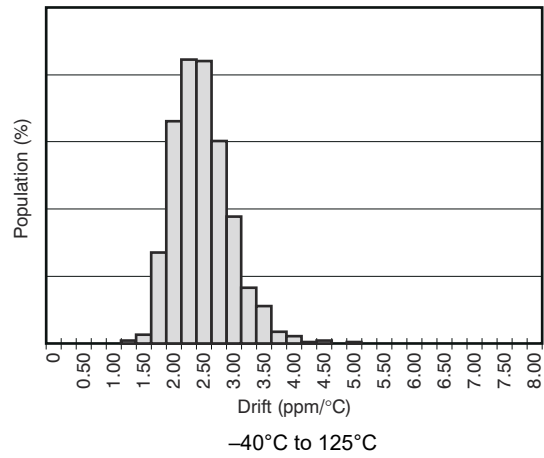
Figure 7-2. Temperature Drift
