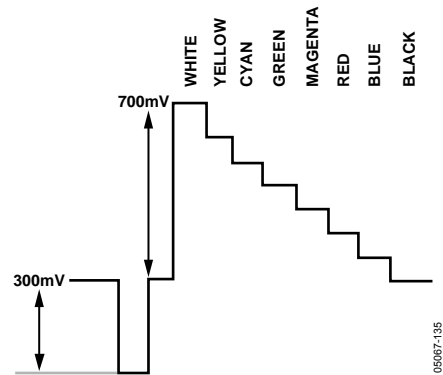
Figure 135. Y Levels—NTSC
