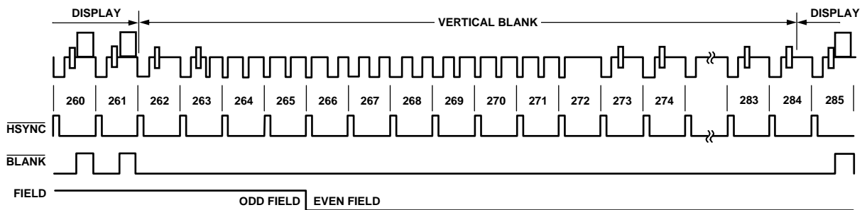
Figure 120. SD Timing Mode 3 (NTSC)
