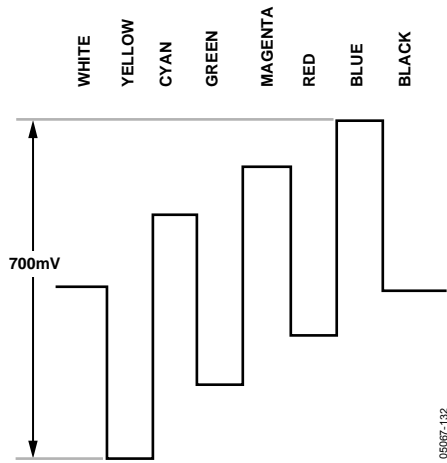
Figure 132. Pb Levels—PAL
